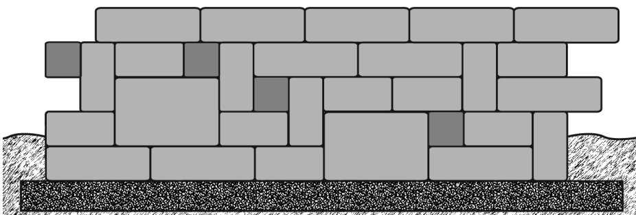
Random Pattern: 3.36 blocks per face foot. Each 20" x 60" section uses 30 blocks. *The dark grey blocks represent cuts.
