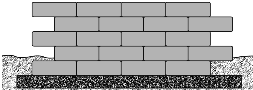
Running Bond Pattern: 3 block per face foot. Each 20" x 48" section uses 20 blocks.
